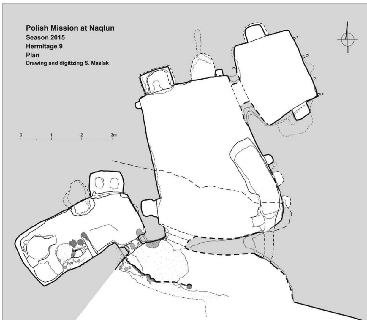
Fig. 1. Hermitage EE.06. The plan (drawing and digitalisation by S Maślak, archive of PCMA).
